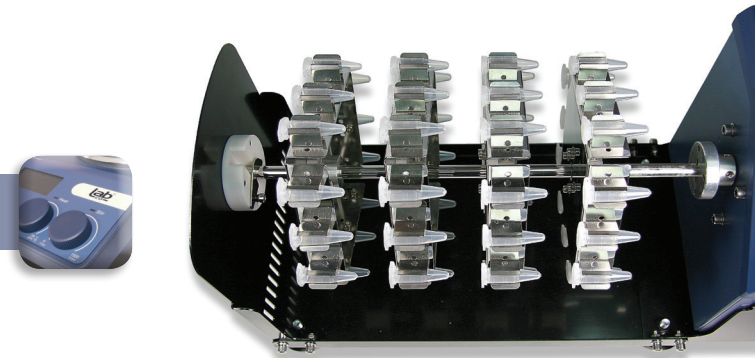
400.104.045 Horizontal Attachment for 1.5mL x 48 Micro Tubes (tubes not included)
